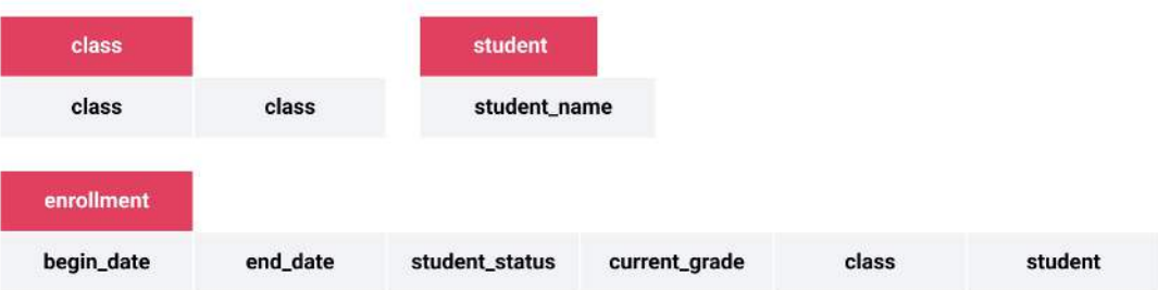
Figure 3: Relational Representation
