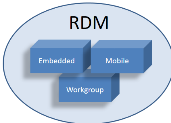
Figure 1: RDM Packages
