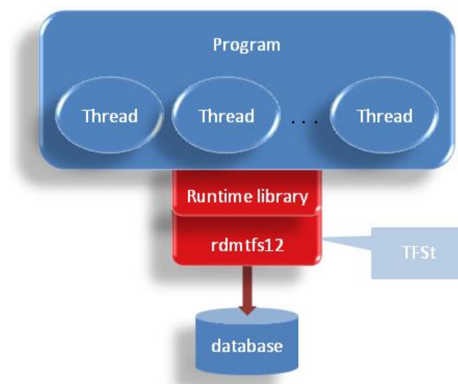
Figure 4: TFSt Functions called by Runtime
