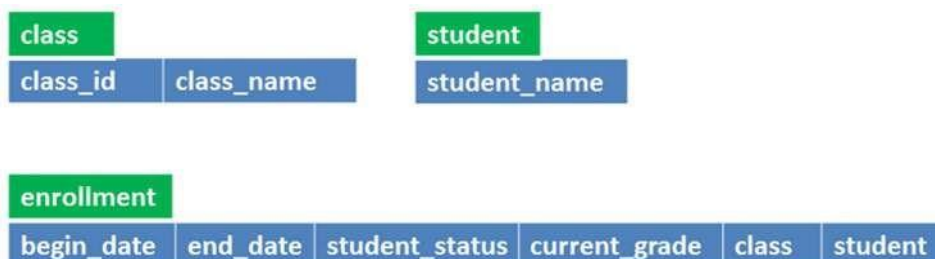
Figure 3: Relational Representation
