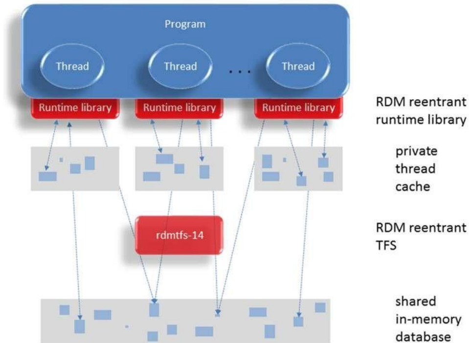
Figure 8: Single-Process, Multiple Threads Configuration
