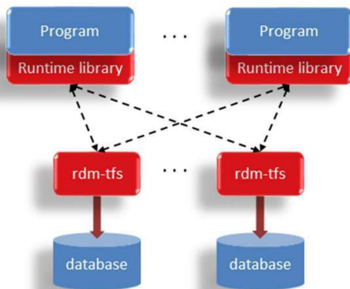
Figure 5: Runtime Library/TFS Configuration
