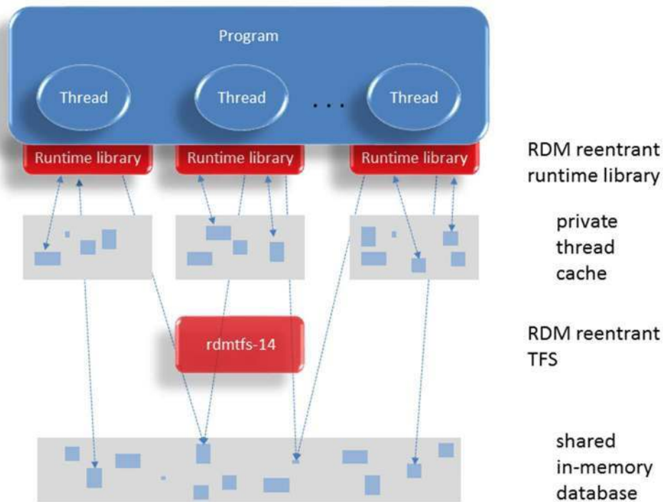
Figure 7: Single-Process, Multiple Threads Configuration
